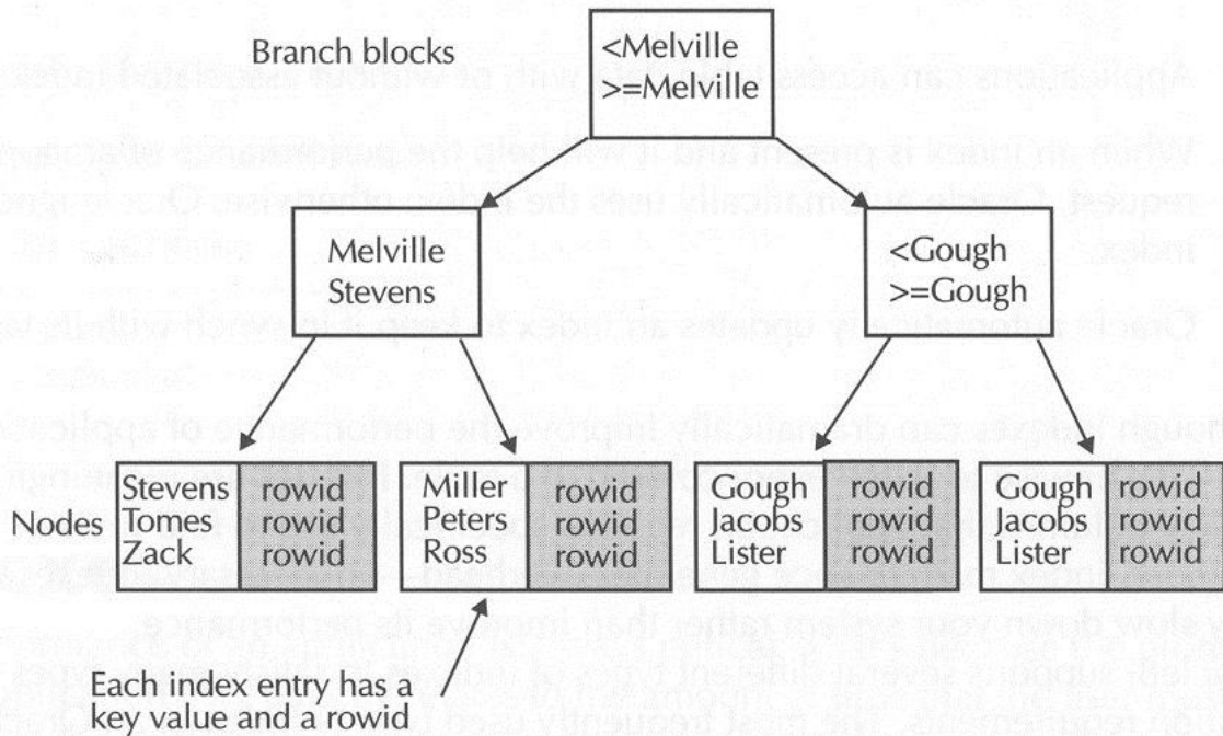
FIGURE 7-4. A B-tree index
